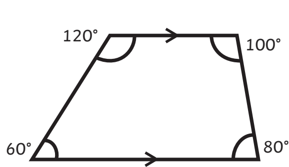
Irregular Trapezium
