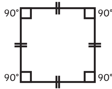
Square
