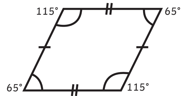
Parallelogram
