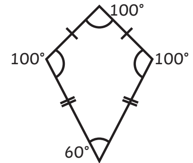
Kite
